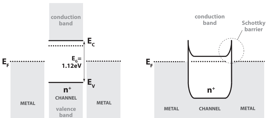
Figure 6: Schematic band diagram of a \Psi -MOSFET with n-channel in silicon (work function of metal larger than that of semiconductor: \phi_m > \phi_s ), in the case of separated (left figure) and continuous (right figure) areas in the device. E_V and E_C denote the band edges of valence and conductance band, respectively, other indices as before.
