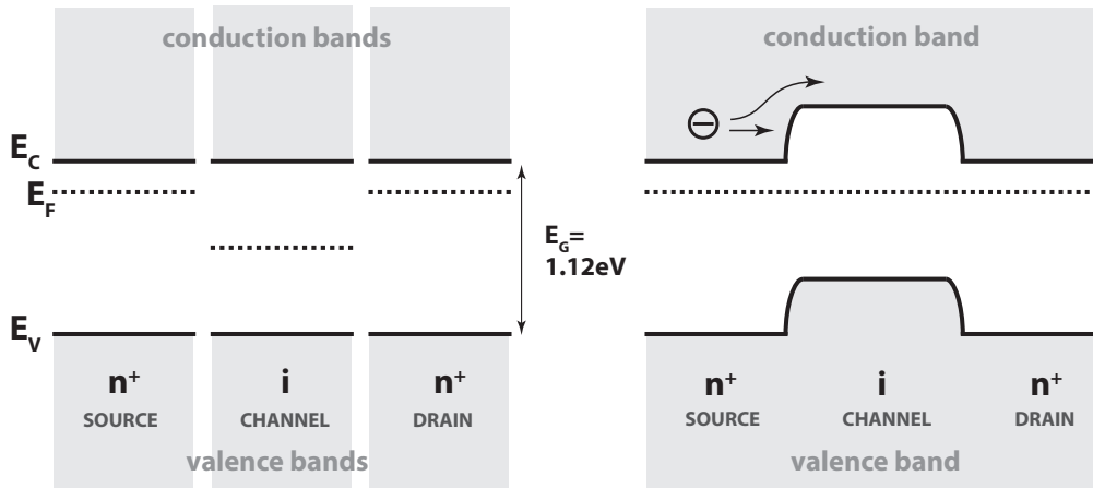
Figure 5: Schematic band diagrams of a MOSFET in silicon, in the case of separated (left figure) and continuous (right figure) areas in the device. E_V and E_C denote the band edges of valence and conduction band, respectively, E_F is the Fermi energy. In case of an average n-type doping ( = n^+ ), E_C - E_F is approx. 40...60 meV, 'i' denotes undoped ( = intrinsic) areas. Here, the Fermi level is in the middle of the bandgap.
