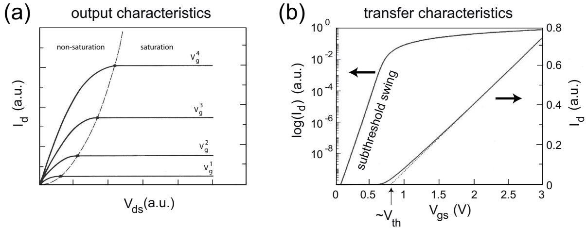
Figure 4: Output (a) and transfer (b) characteristics of a MOSFET.
