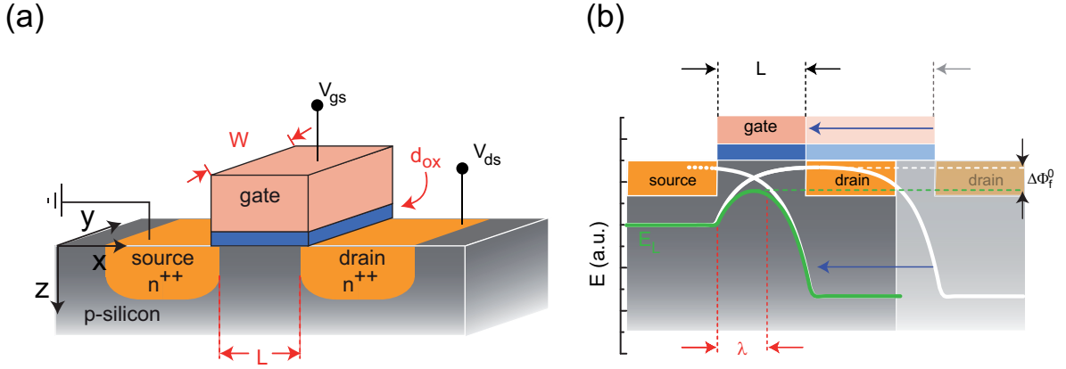
Figure 1: (a) Schematics of a conventional bulk-Si MOSFET. (b) Illustration of the appearance of short channel effects in a scaled device: the white line represents the conduction band along current transport direction in a long-channel device. In a device suffering from SCE, the source-channel and channel-drain p-n junctions overlap leading to a lowering of the potential barrier in the channel (green solid line). As a result, devices exhibiting SCE show an exponentially increased off-state leakage leading to a drastic increase of power consumption and eventually a loss of the ability to switch the device.
