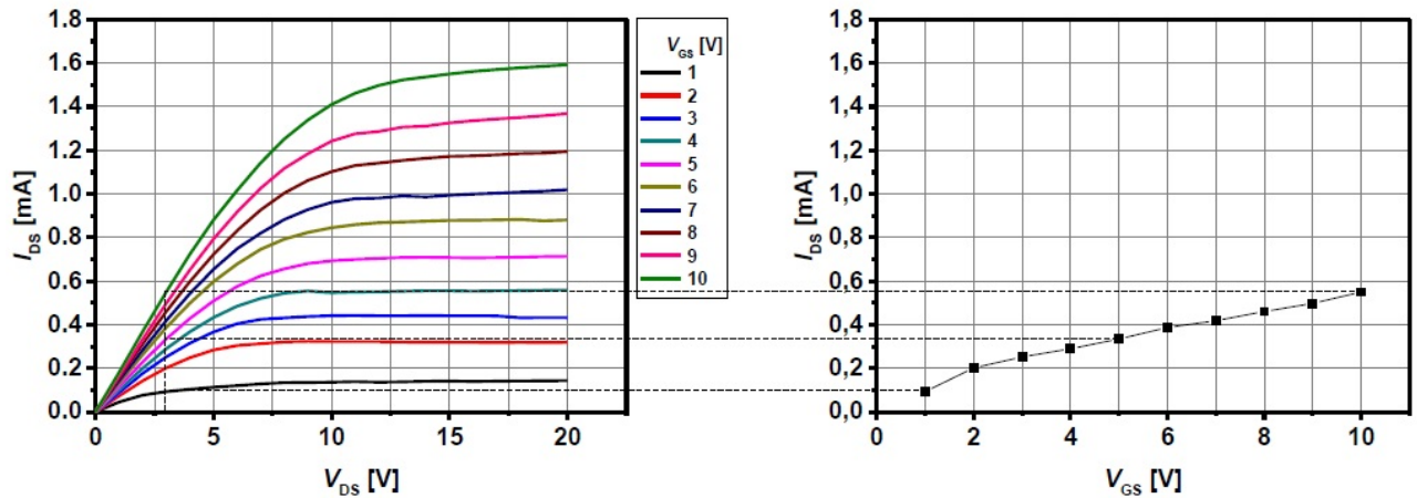
Figure 13: Output and derived transfer characteristics
