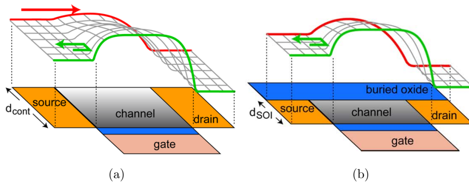
Figure 3: Two-dimensional conduction band profiles for MOSFET devices based on (a) bulk-silicon and (b) silicon-on-insulator substrates.
