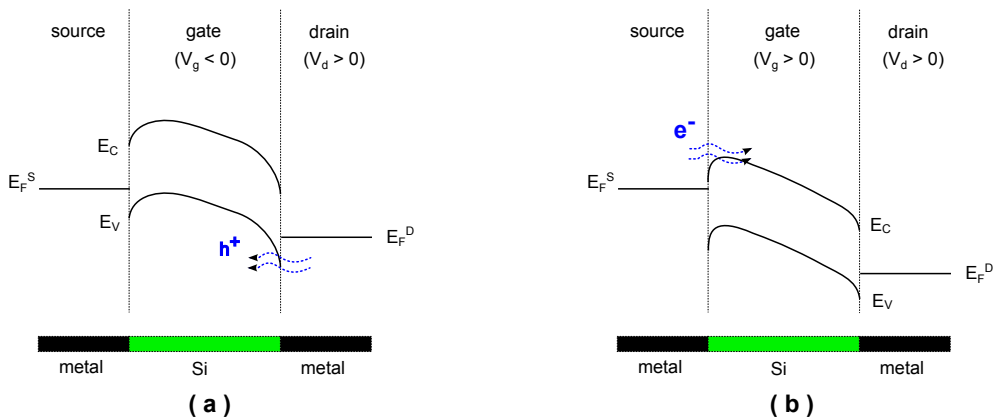
Figure 9: A \Psi -MOSFET with p-type silicon. If the gate is biased with negative voltage, the channel stays as a p-type channel, holes are injected from drain to channel with a positive drain voltage applied to the drain electrode (a) and if the gate is biased with sufficient positive voltage, the channel is then inverted into an n-type channel, thermally excited electrons can then pass the source-channel junction with an additional positive voltage applied to the drain electrode (b).
