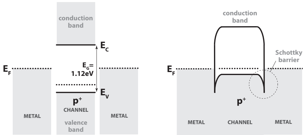
Figure 7: Schematic band diagram of a \Psi -MOSFET with p-channel in silicon (work function of metal smaller than that of semiconductor: \phi_m < \phi_s ), in the case of separated (left figure) and continuous (right figure) areas in the device. E_V and E_C denote the band edges of valence and conductance band, respectively, other indices as before.
