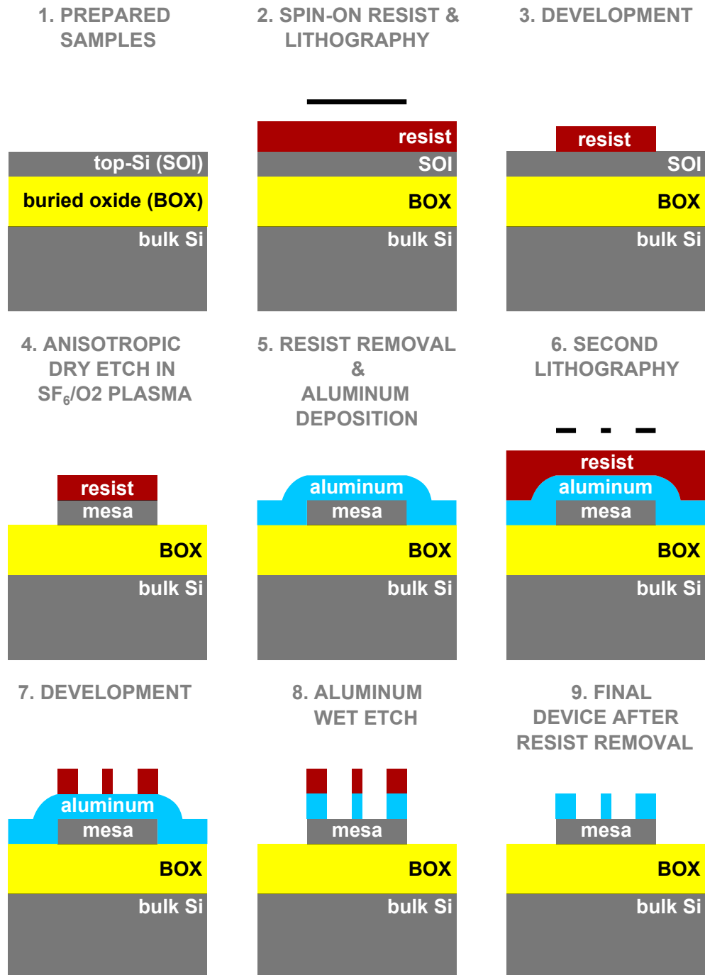
Figure 11: Schematics of device fabrication process flow.
